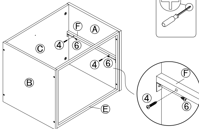
Screw 1
