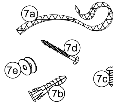
Safety strap kit Qty: 1
