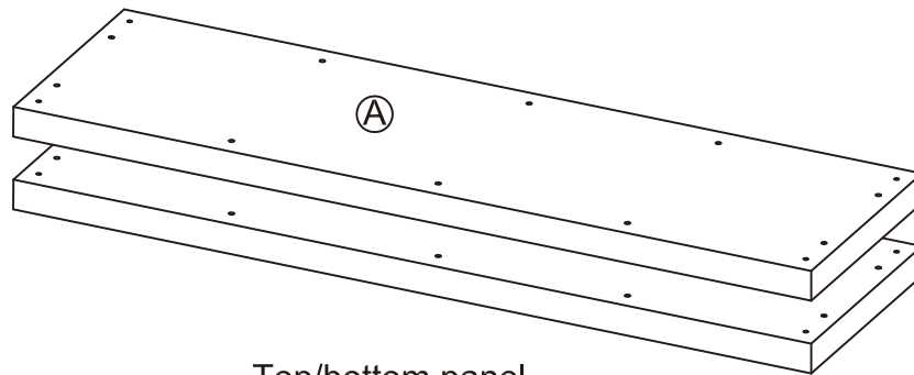
Top/bottom panel
