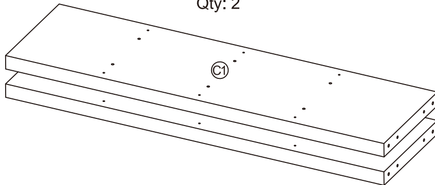
Side panel
