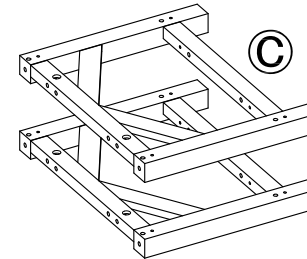
Side frame (Qty: 2)
