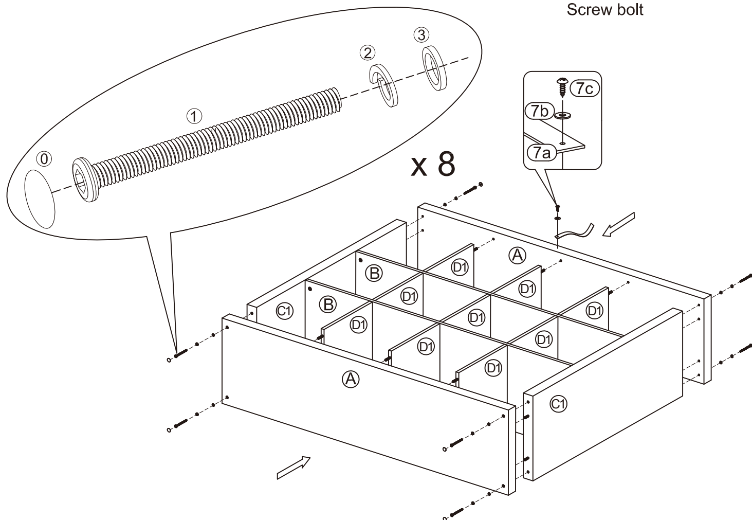
Screw bolt
