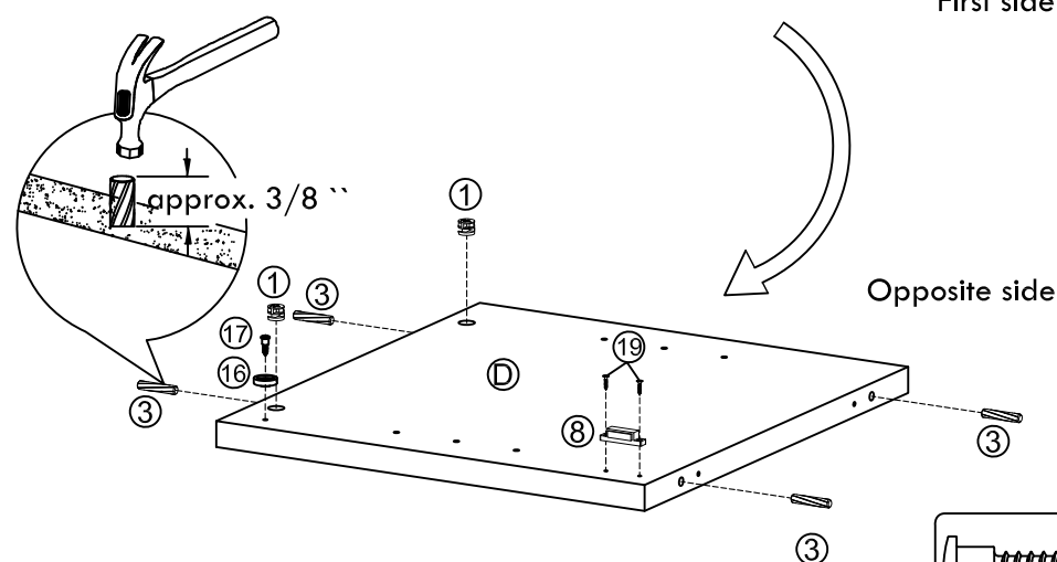
First side
