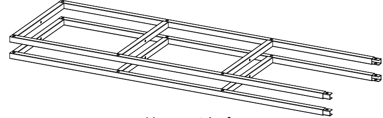
Upper side frame (Qty: 2)
