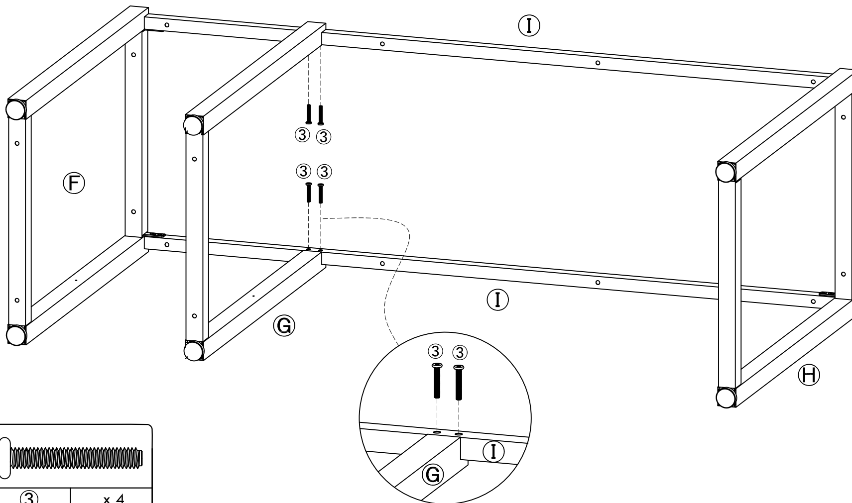
Screw Bolt 3
