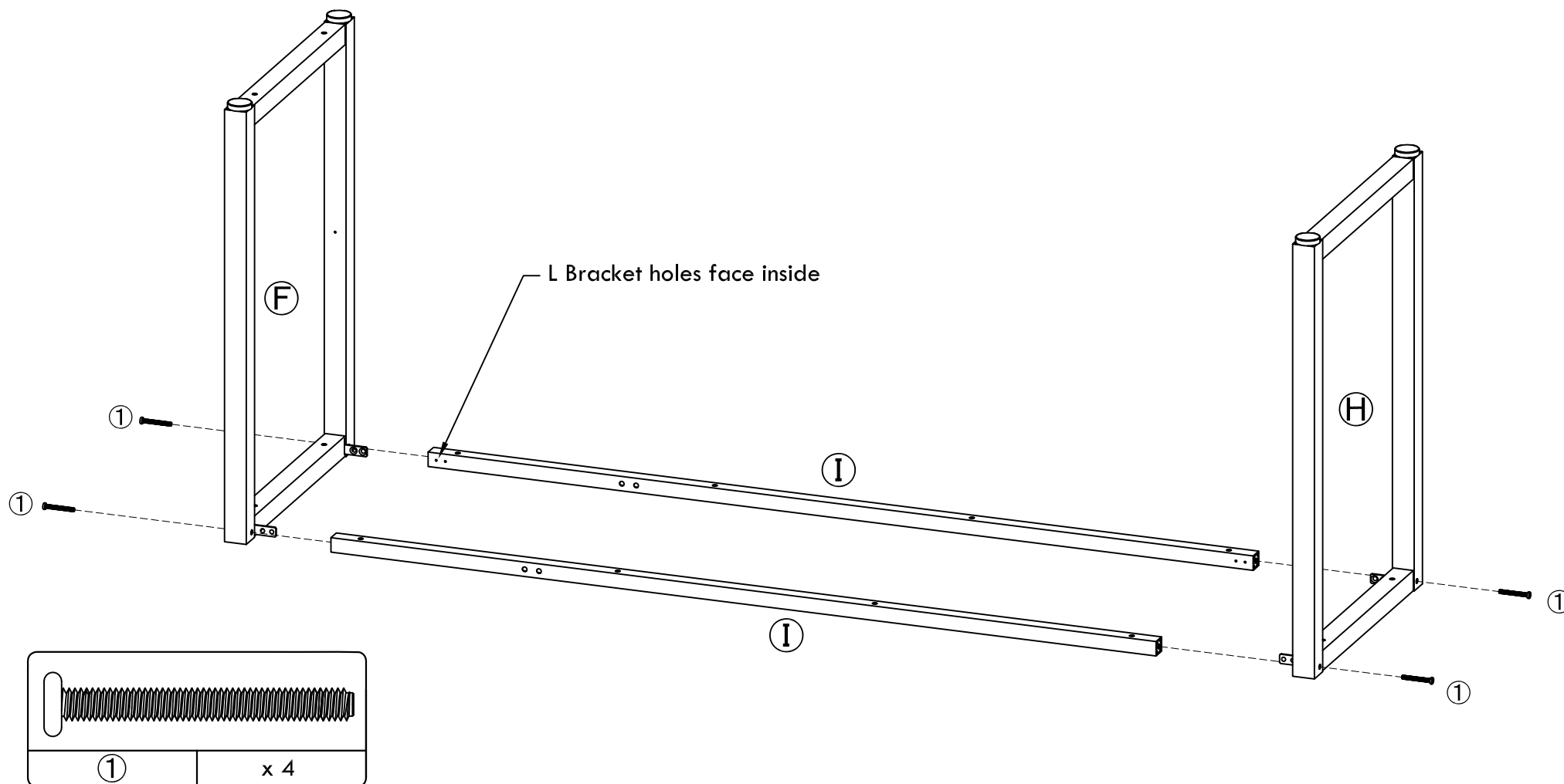
Screw Bolt 1
