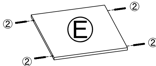
“E” WITH LONG DOWELS IN BOTH ENDS
